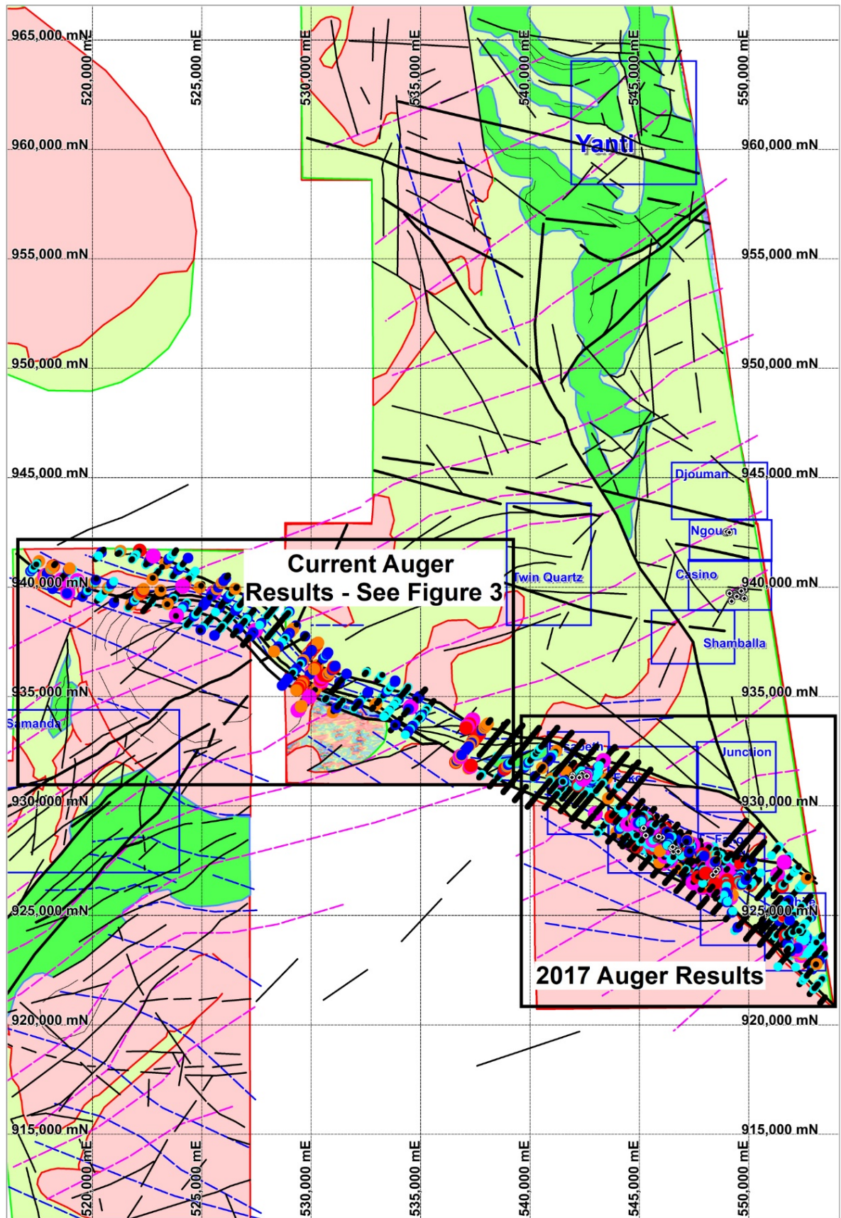
Figure 2: Bondoukou Project – All auger drilling over Awari Shear showing previously reported (2017) results and the current reporting area.
