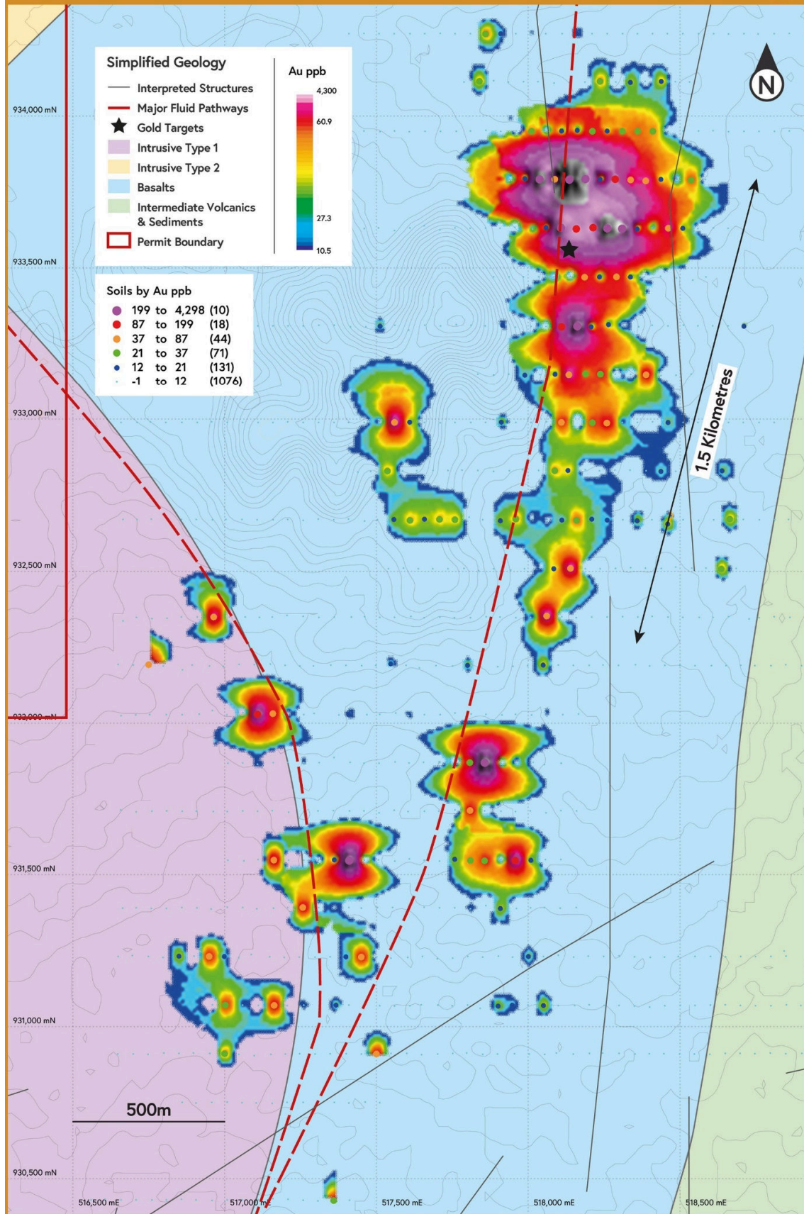
Figure 4: Samanda East gold in soils over simplified geology.
