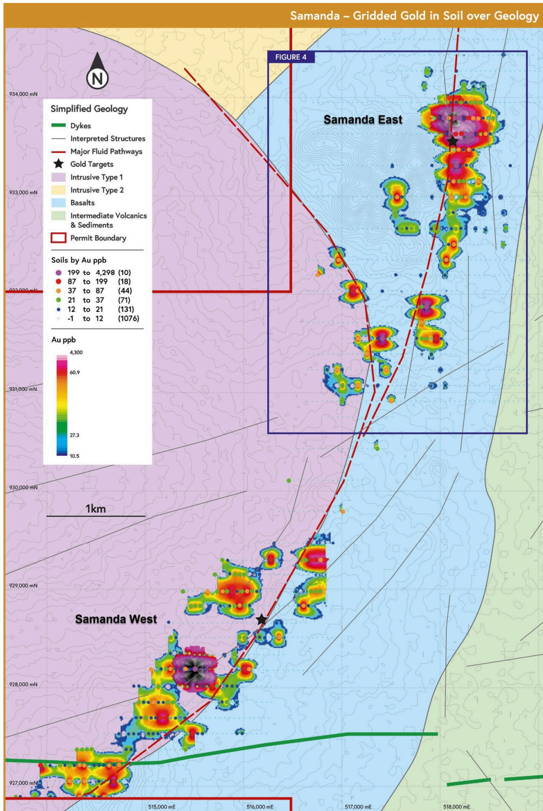
Figure 3: Samanda soil results over simplified geology, red dashed lines are interpreted major structures/fluid pathways. 2 main 3km long trends defined. After infill sampling Samanda East (figure 4), has presented as a standout and robust anomaly.
