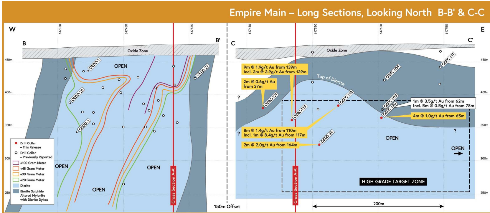
Figure 4: Long Sections B-B' (Empire Main) and C-C' (Empire Gap) – looking North, The Empire Gap long section is 150m south of the Empire Main section.
