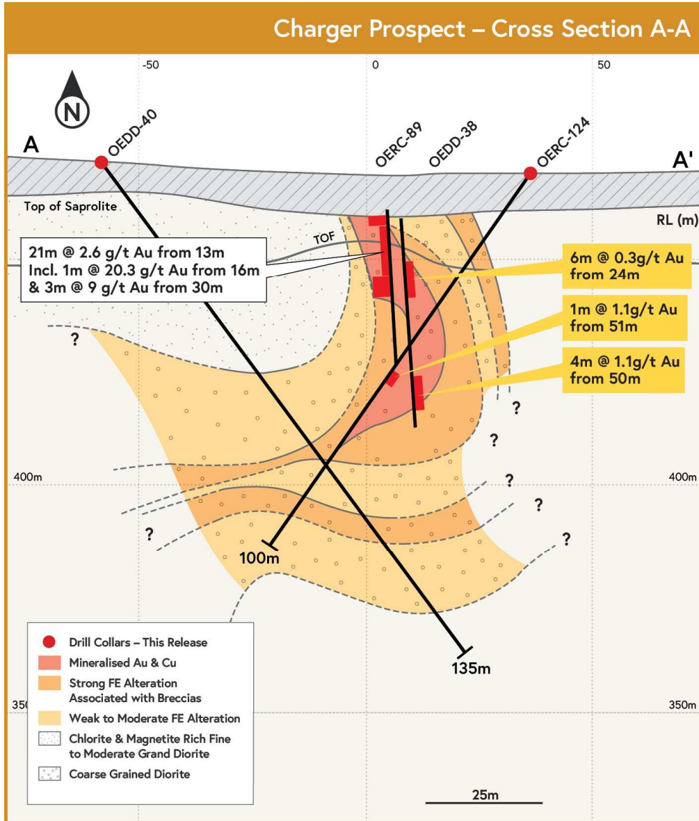
Figure 7: Charger cross section, looking West.
