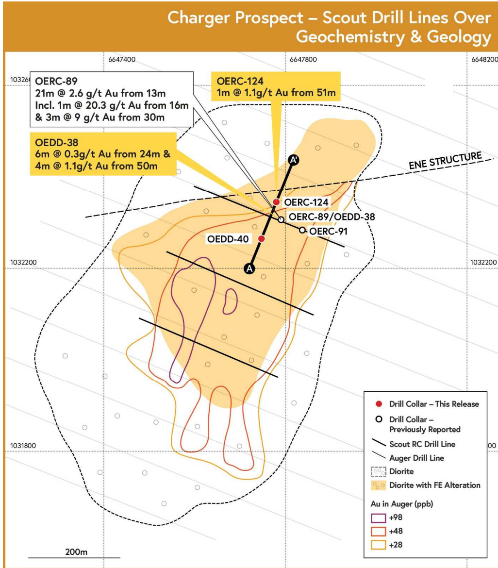
Figure 6: Charger drill lines over simplified geology. Red collars are reported in this release.
