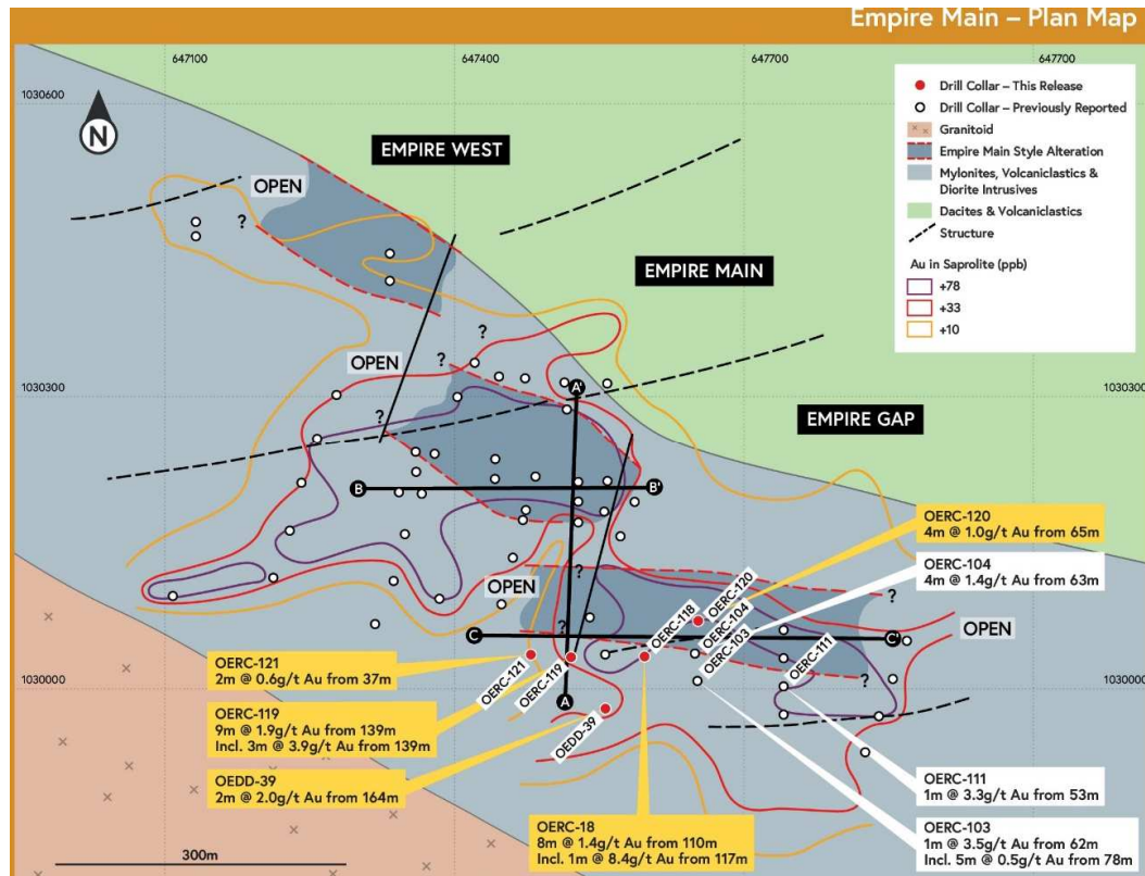
Figure 3: Plan Map - Empire showing new 'Gap Offset' drillholes (red collars) over geology and auger geochemistry contours. Long Section B-B'/C-C' (Figure 4) and Cross section A-A' (Figure 5) lines are shown.
