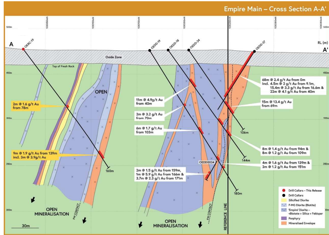
Figure 5: Cross Section looking west for hole OERC-119 shown with the Empire Main drill holes 150m metres to the North.
