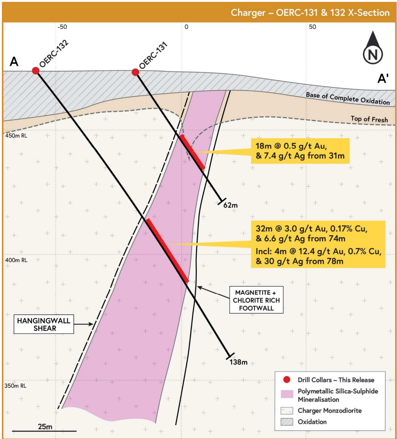
Figure 3: Charger cross section A-A' from figure 2 showing drillholes OERC-131 and OERC-132
