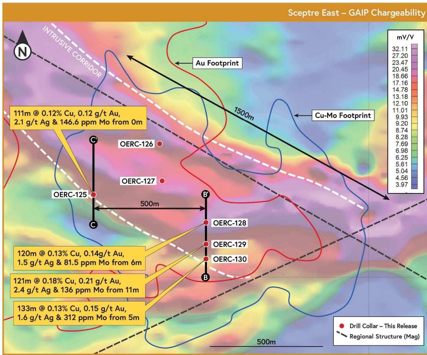
Figure 4: Sceptre East drill hole locations over IP chargeability image
