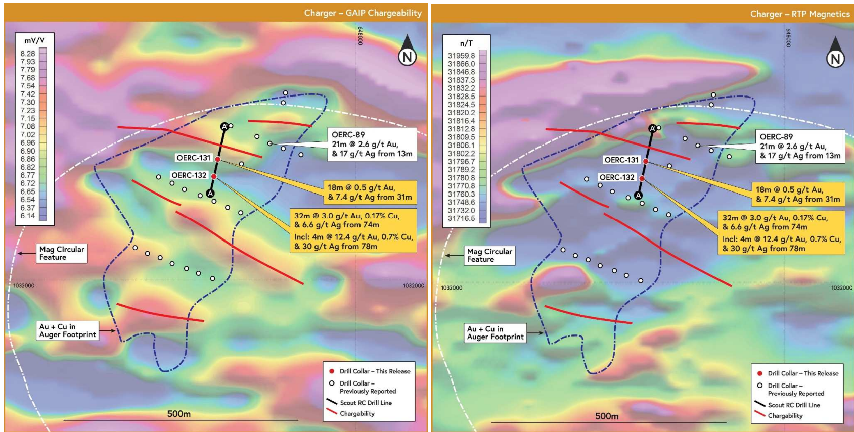
Figure 2: Charger drilling over IP chargeability (left) and RTP magnetics (right). Drill intercepts from this release are in yellow boxes.
