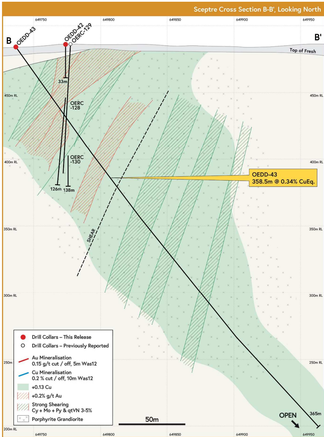
Figure 6: Sceptre East Cross Section B-B' - Hole OEDD-43.
