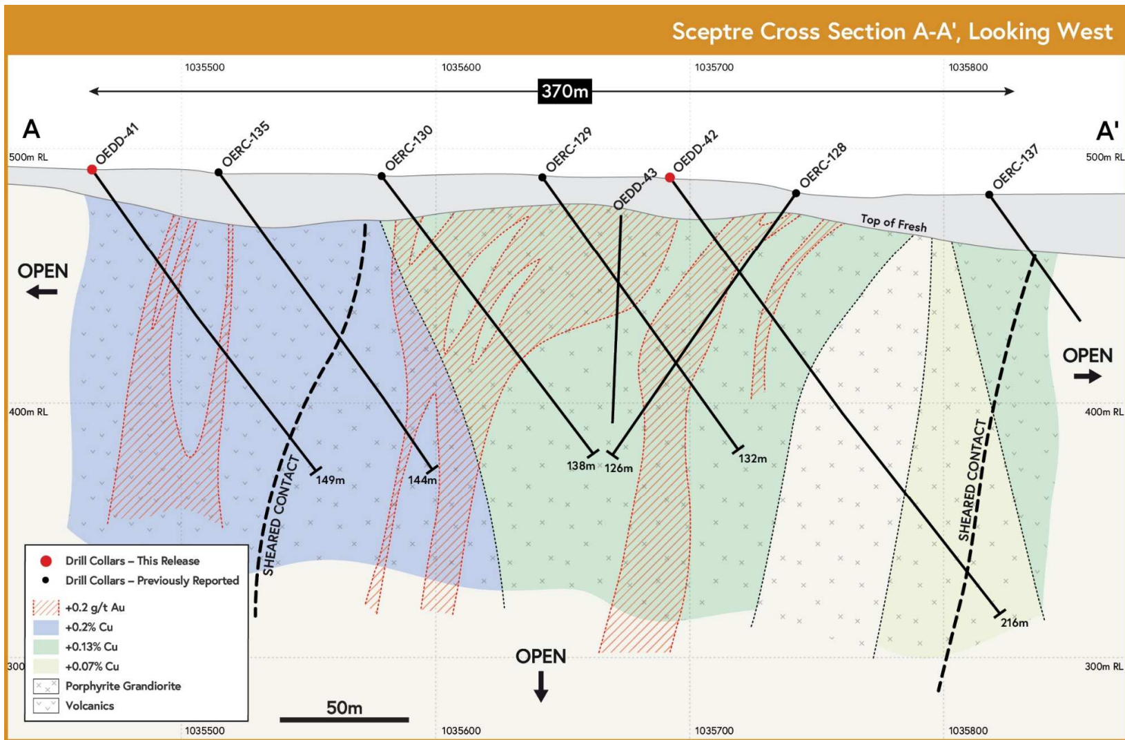
Figure 5: Sceptre East drill section A-A'.
