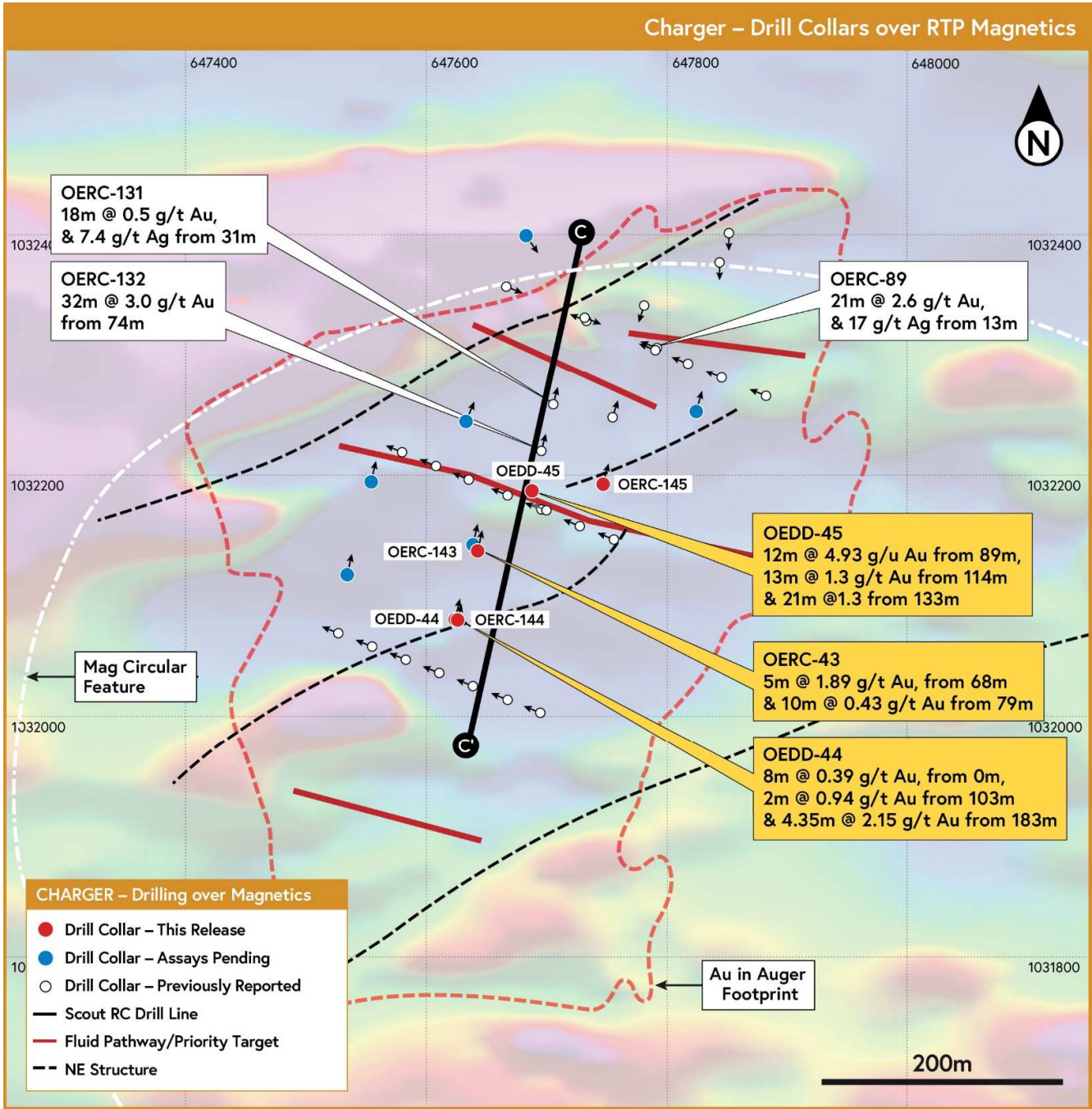
Figure 2: Charger drilling over RTP magnetics. Drill intercepts from this release are in yellow boxes.
