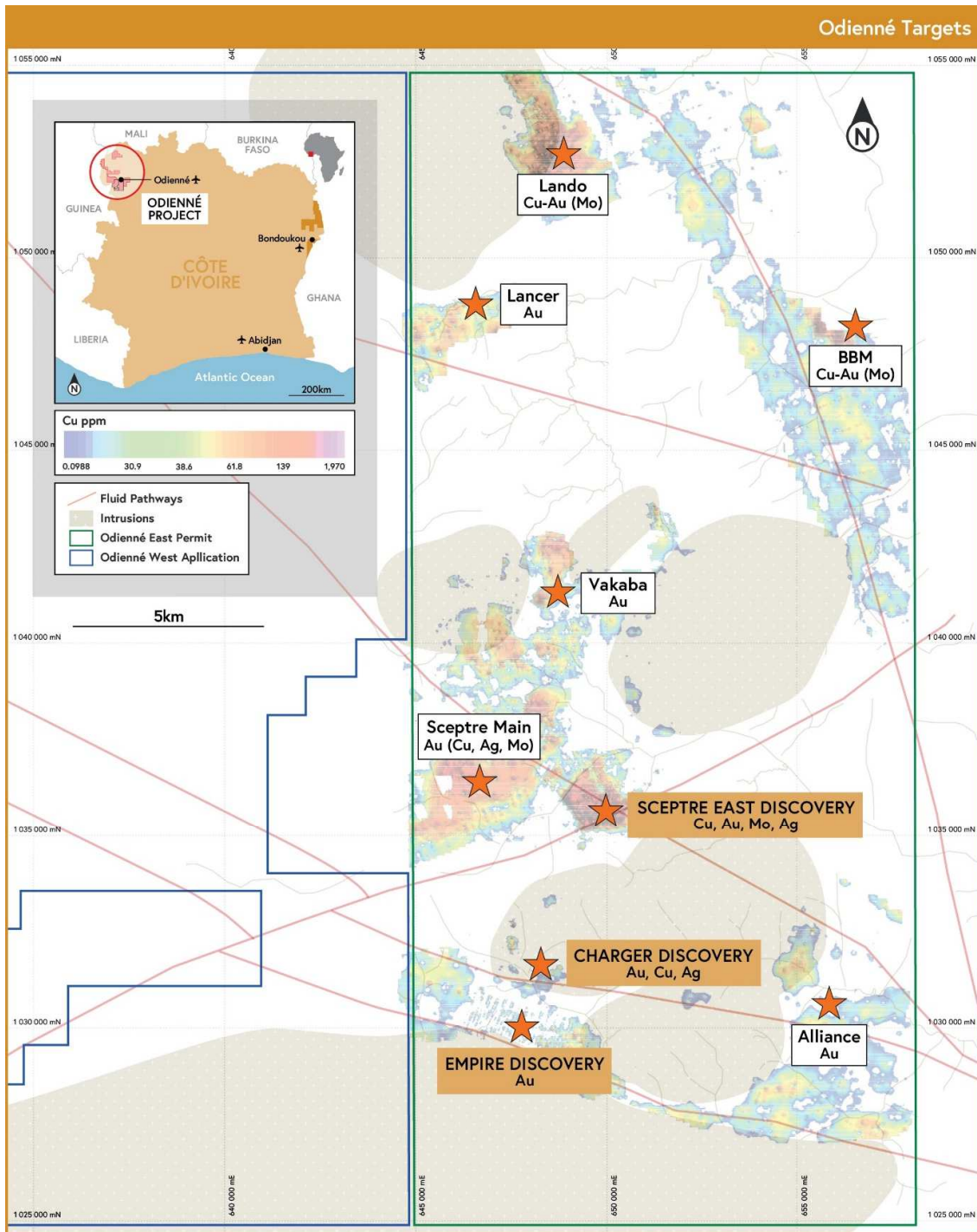
Figure 1: Odienné Project, Prospect Locations. Drilling at Sceptre East and Charger (red boxes) are reported in this release.
