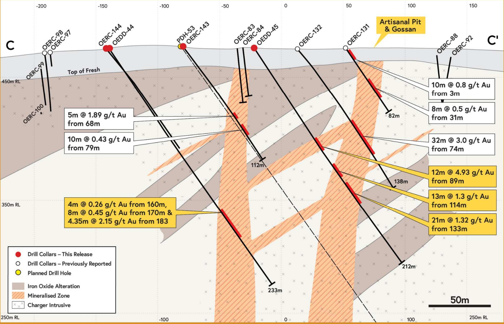
Figure 3: Charger cross section C-C' from figure 2
