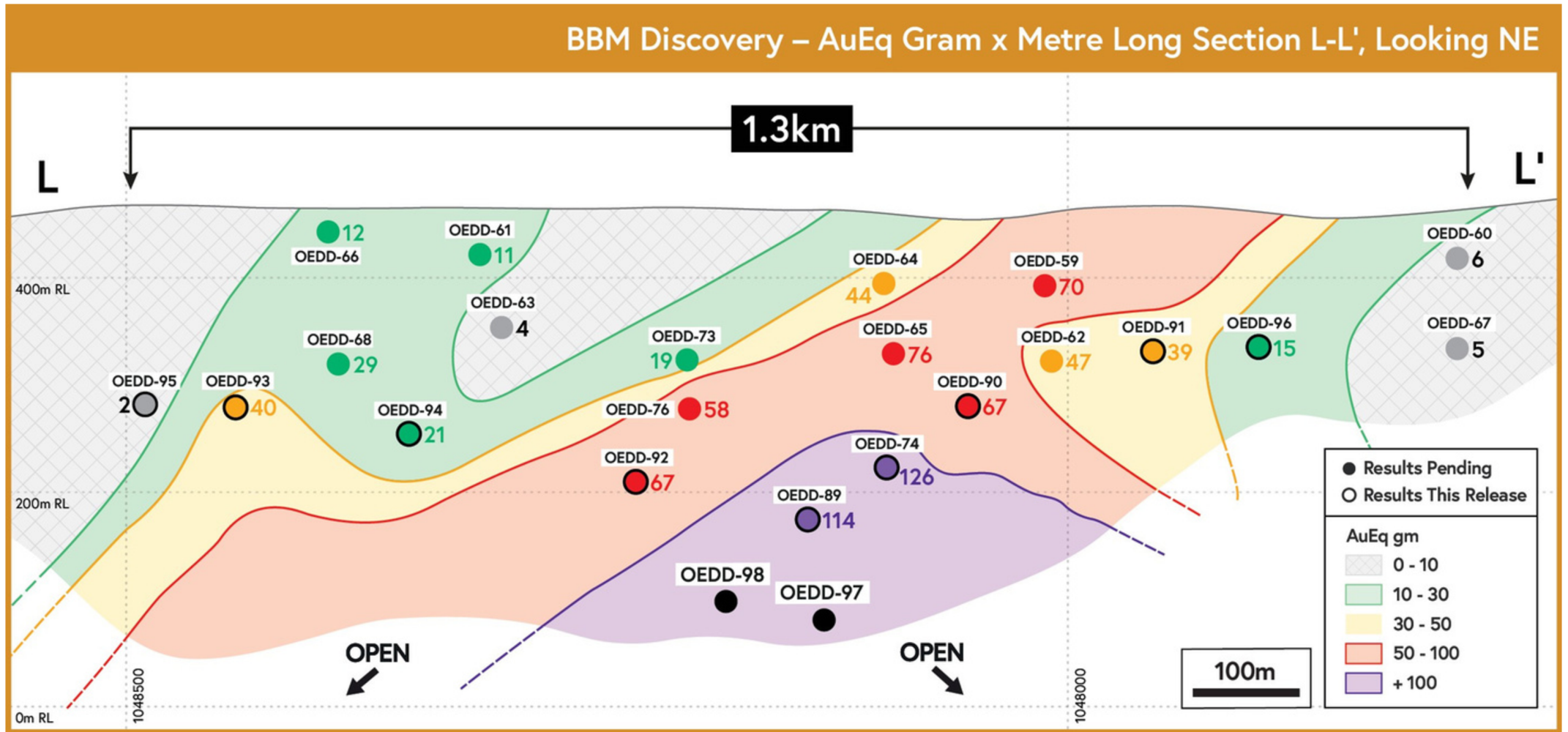
Figure 3: Long section looking NE through BBM drilling, depicting contours of gold equivalent grams x metres. The section shows the northwest plunge of the high grade mineralization and an increase in grade with depth. Mineralisation remains open down dip and plunge, as well as other plunge targets within this 1.3km zone.
