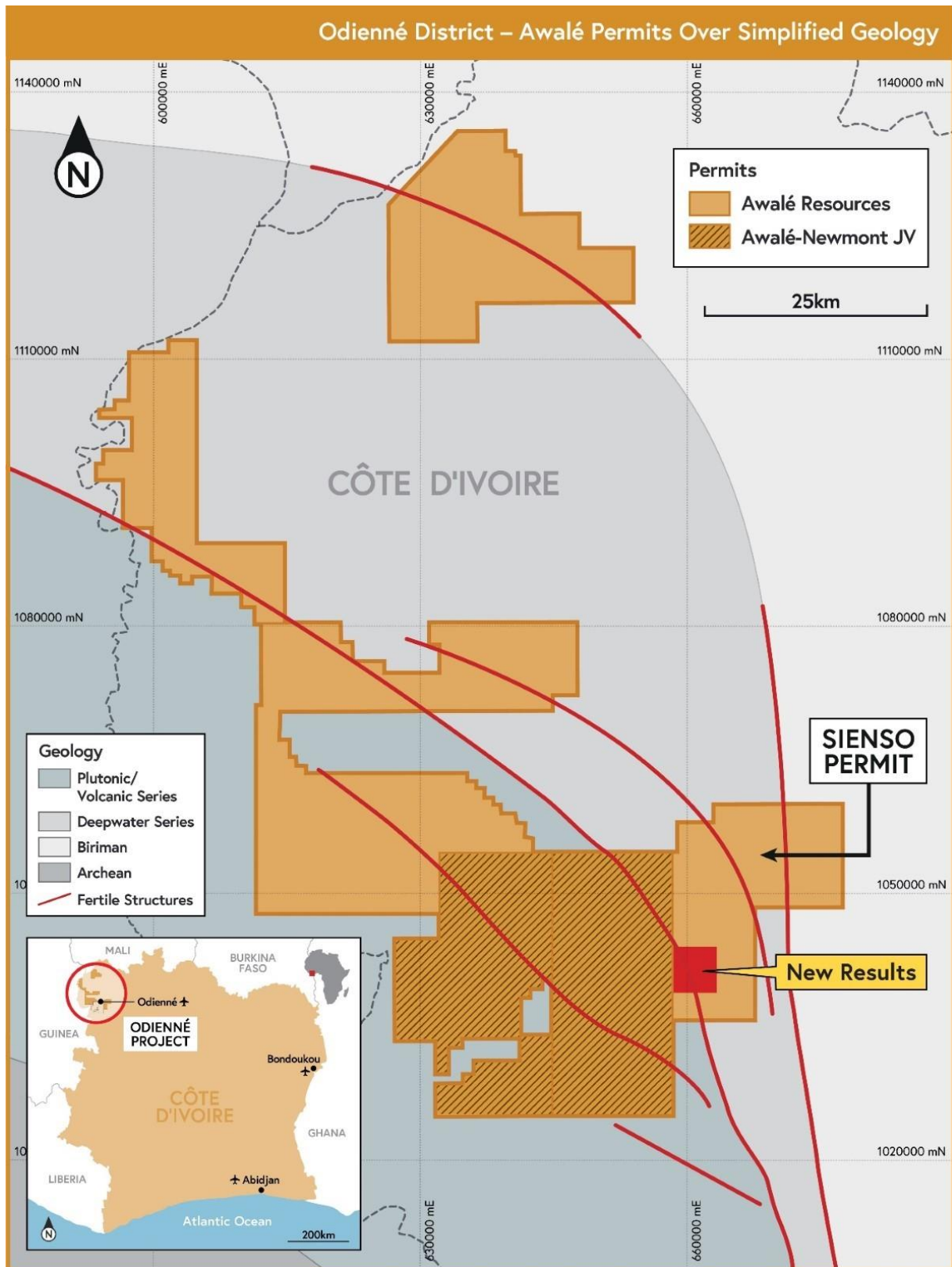
Figure 1: Awalé Permits in NW Côte d'Ivoire – Showing new geochemistry area as red box in Awalé's 100%-owned Siensou permit.
