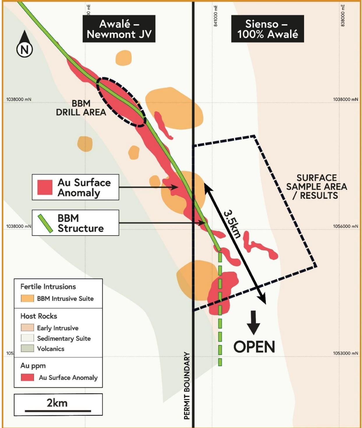
Figure 2: New 3.5km long > 37 ppb Gold footprint in Awalé’s 100%-owned Sienso Permit. A direct extension of the BBM discovery.
