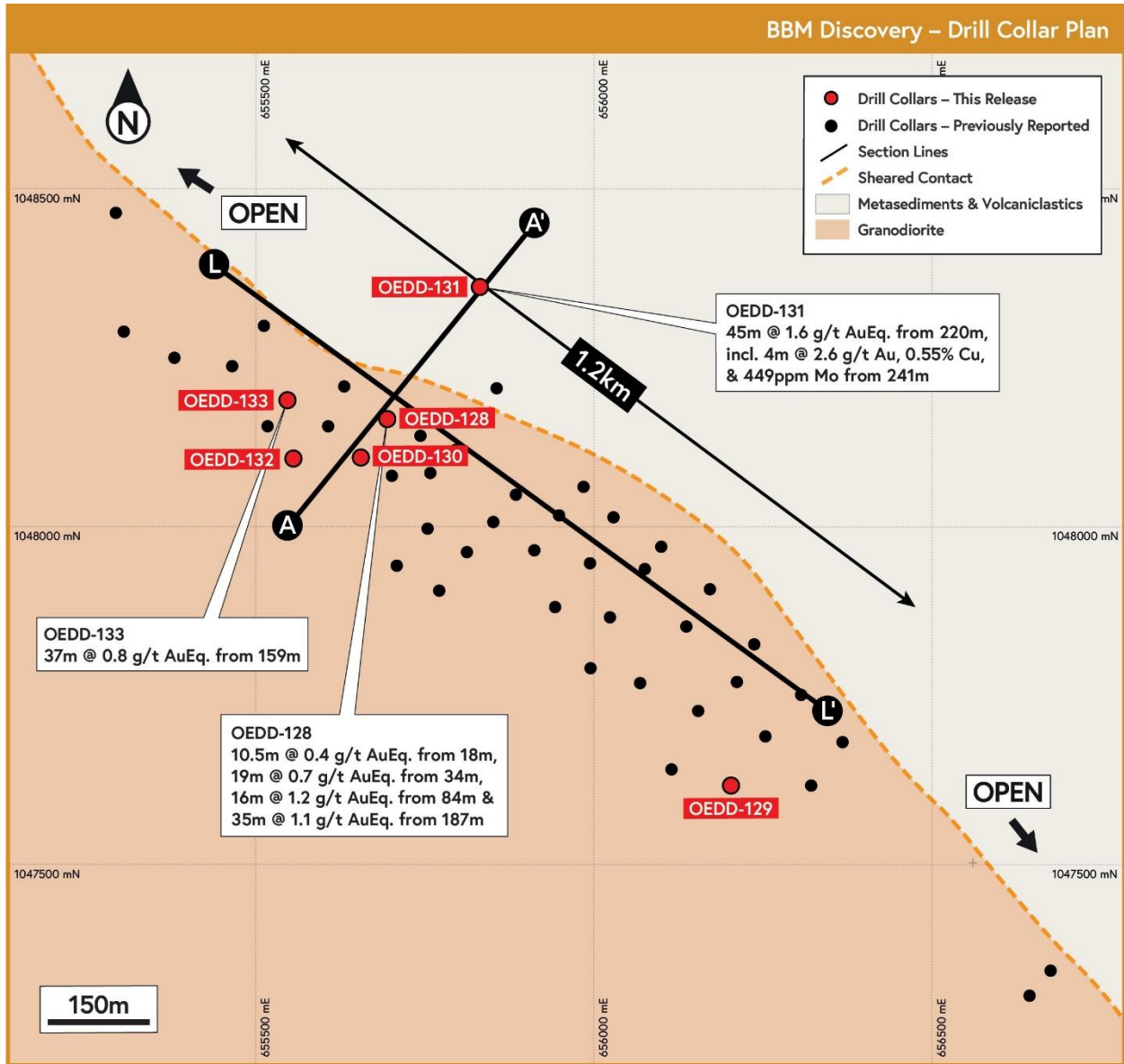
Figure 1: BBM Drill Collar Plan, shown over simplified geology.
