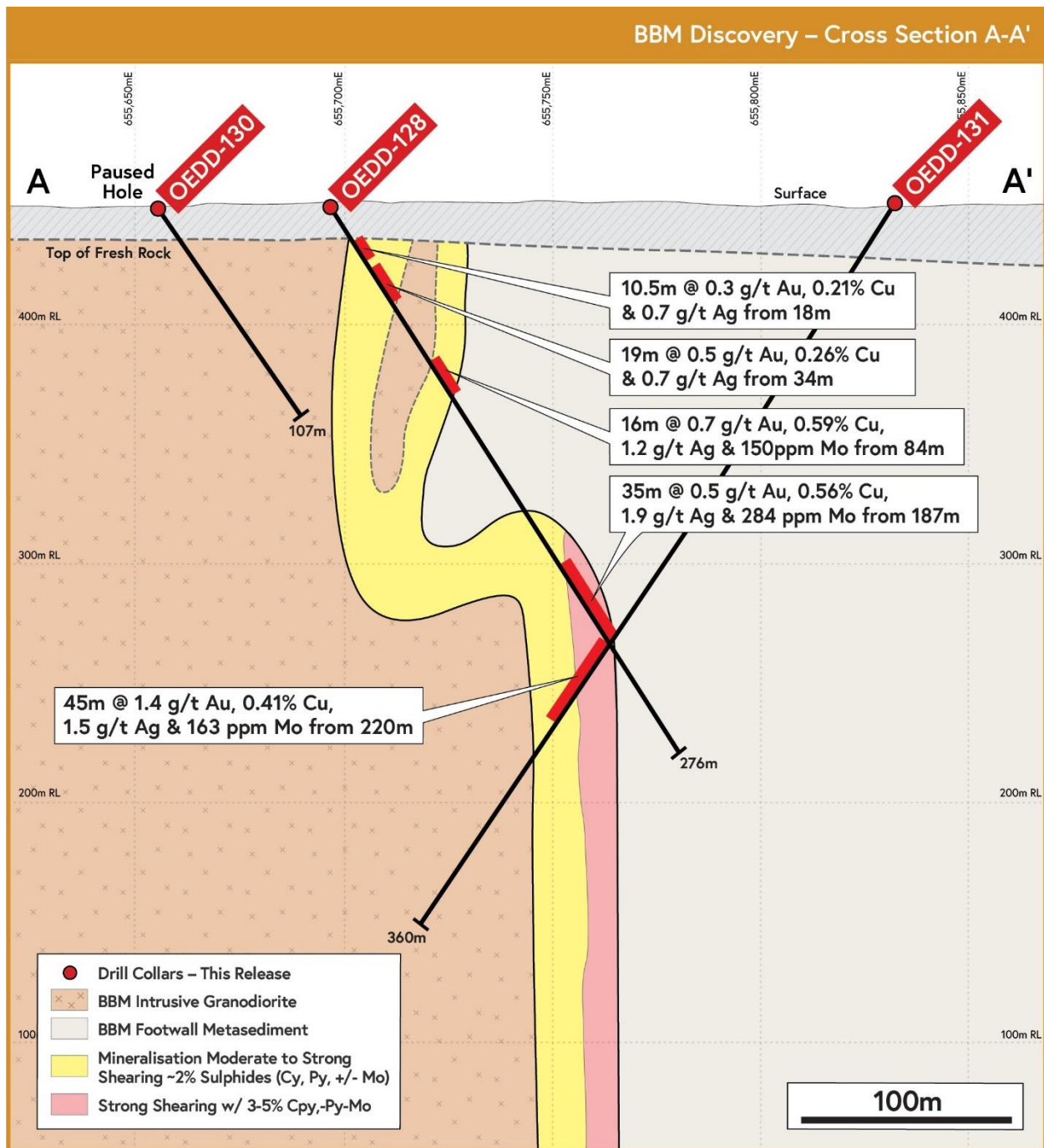
Figure 2: Drill Section A-A' through holes OEDD-128, OEDD-130, OEDD-131, reported in this release. Looking toward the NW 50m Window.
