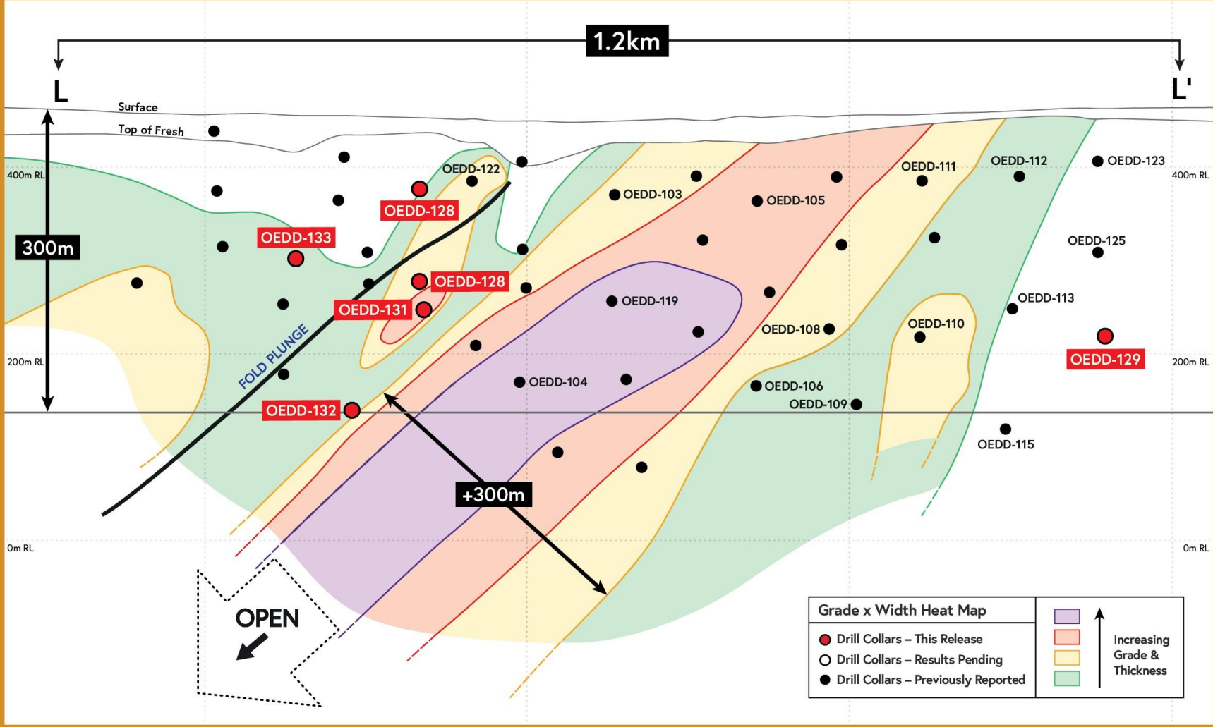
Figure 3: BBM Long Section L-L', showing a grade width heatmap, along with all planned and drilled holes from this drill program.
