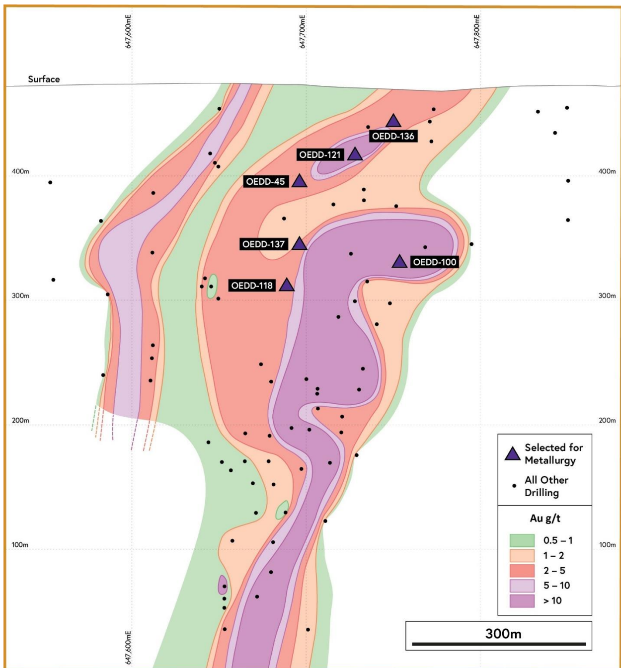
Figure 2: Charger Deposit – Long section showing the location of drill holes selected for metallurgical testwork (purple triangles).
