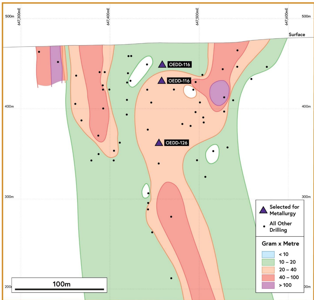
Figure 3: Empire Deposit – Long section showing the location of drill holes selected for metallurgical testwork (purple triangles).
