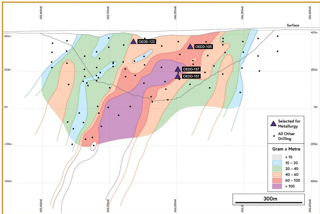
Figure 1: BBM Deposit – Long section showing the location of drill holes selected for metallurgical testwork (purple triangles).
